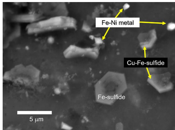
Figure 3. Electron backscattered (BSE) photomicrograph of multiple randomly oriented and broken Fe-sulfide platelets exposed on the floor of a vesicle in Dakhleh glass. Fe-Ni metal grains occur with the sulfides.
