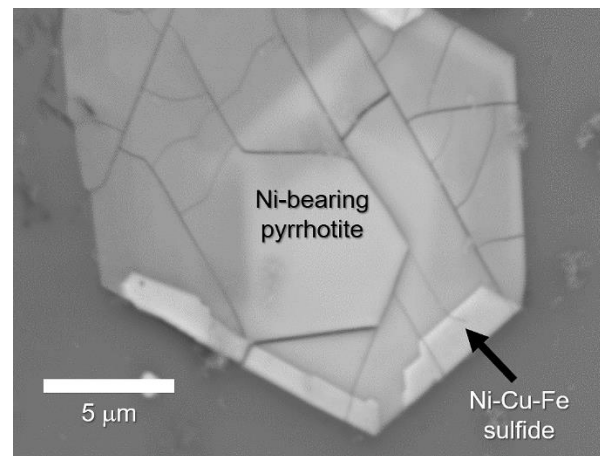
Figure 1. Electron backscattered (BSE) photomicrograph of an Fe-sulfide assemblage exposed on the wall of a vesicle in Pica glass. The rim appears similar to overgrowths of cubanite (CuFe 2 S 3 ) observed on Fe-sulfides from CI meteorites, Stardust samples from Comet 81P/Wild, and experimentally produced sulfides prepared in environments intended to simulate aqueous alteration on comets [9-11].
