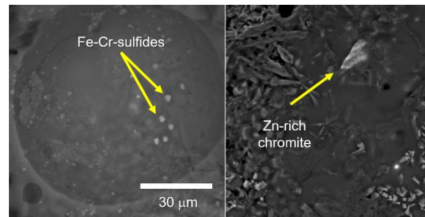
Figure 4. Electron backscattered (BSE) photomicrographs of an Fe-Cr-sulfide grain and a Zn-rich chromite grain exposed in vesicle walls in Edeowie glass.
