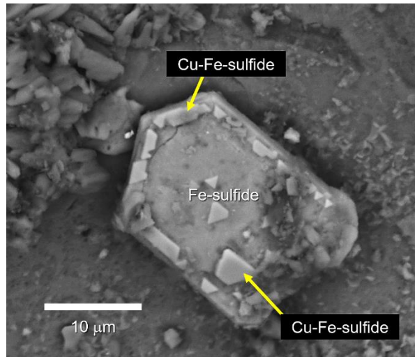
Figure 2. Electron backscattered (BSE) photomicrograph of an Fe-sulfide platelet exposed on the wall of a vesicle in Dakhleh glass. The rim exhibits similar overgrowths to those observed in Pica glass.
